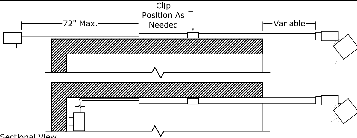
Sectional View Can Be Mounted On Underside Of Cabinetry
